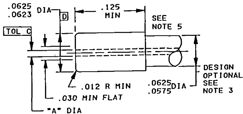
DETAIL W
